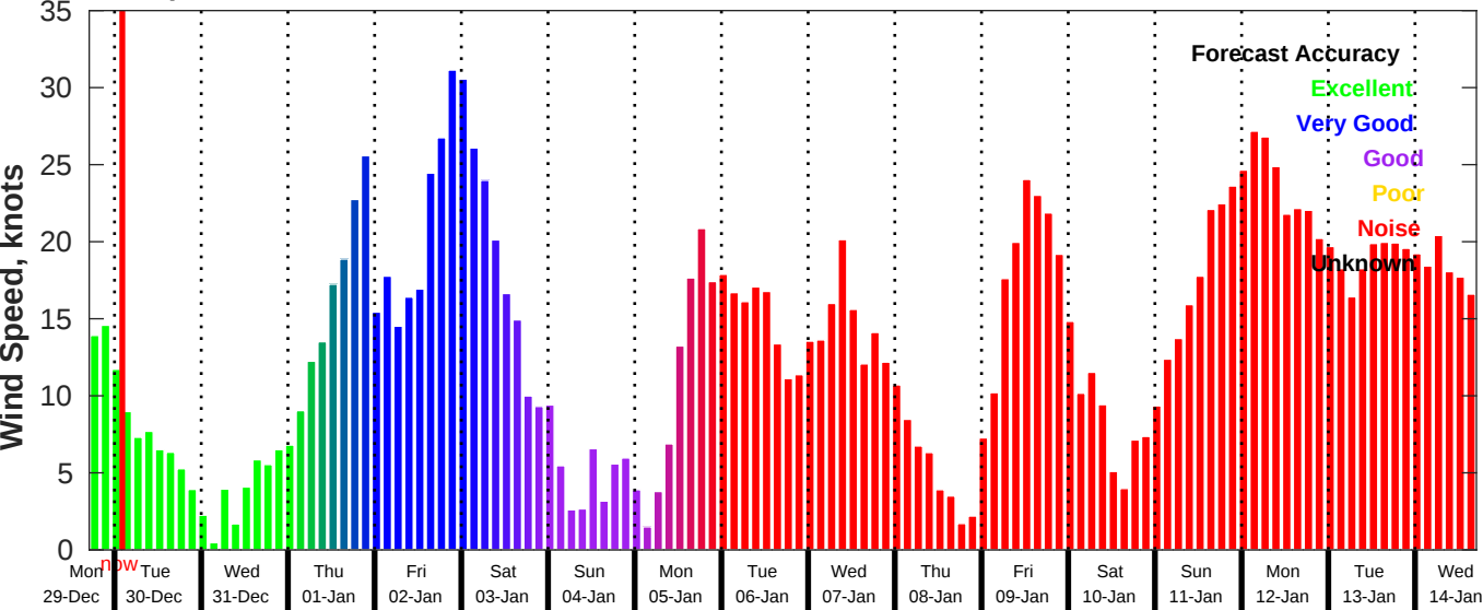
GFS Wind Speed Forecast for NDBC 46059 from 29-Dec-2025 17:00:00 to 14-Jan-2026 17:00:00
