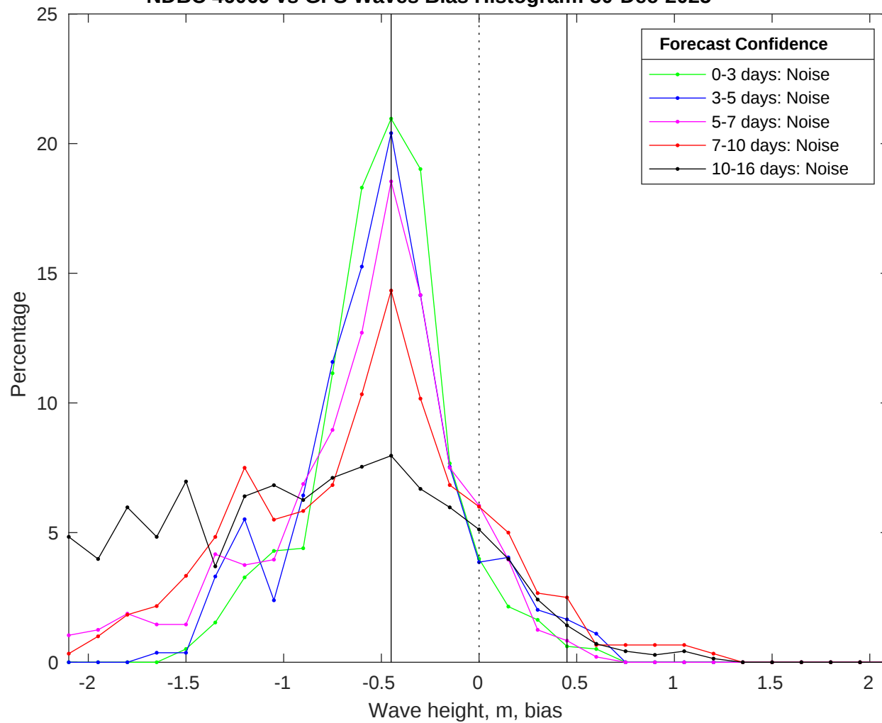
NDBC 46069 vs GFS Waves Bias Histogram: 30-Dec-2025
