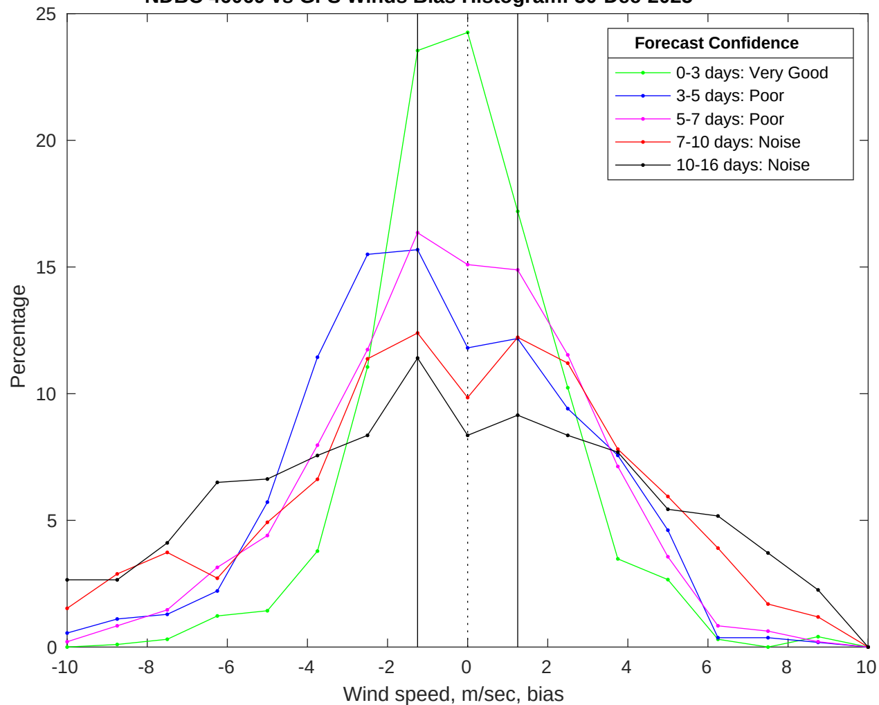
NDBC 46069 vs GFS Winds Bias Histogram: 30-Dec-2025
