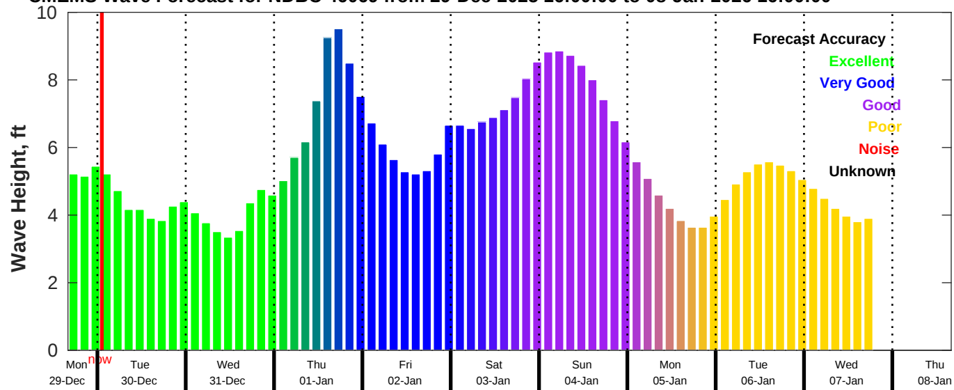
CMEMS Wave Forecast for NDBC 46069 from 29-Dec-2025 16:00:00 to 08-Jan-2026 16:00:00
