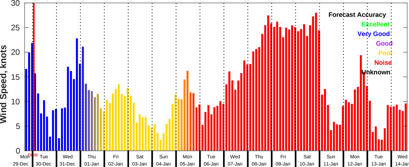
GFS Wind Speed Forecast for NDBC 46069 from 29-Dec-2025 16:00:00 to 14-Jan-2026 16:00:00
