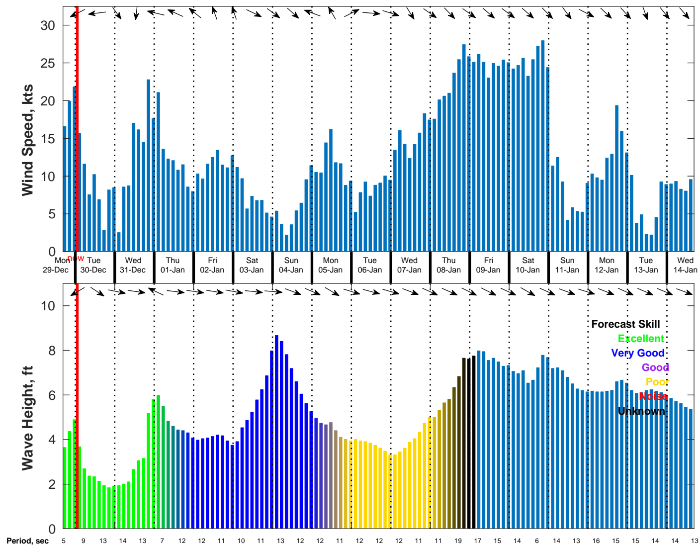
Wind & Wave Forecast for NDBC 46069 from 29-Dec-2025 16:00:00 to 14-Jan-2026 16:00:00
