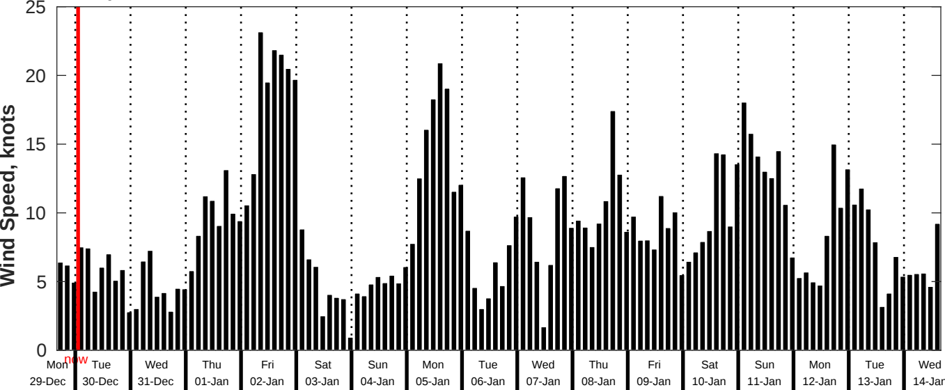
GFS Wind Speed Forecast for NDBC 46215 from 29-Dec-2025 16:00:00 to 14-Jan-2026 16:00:00
