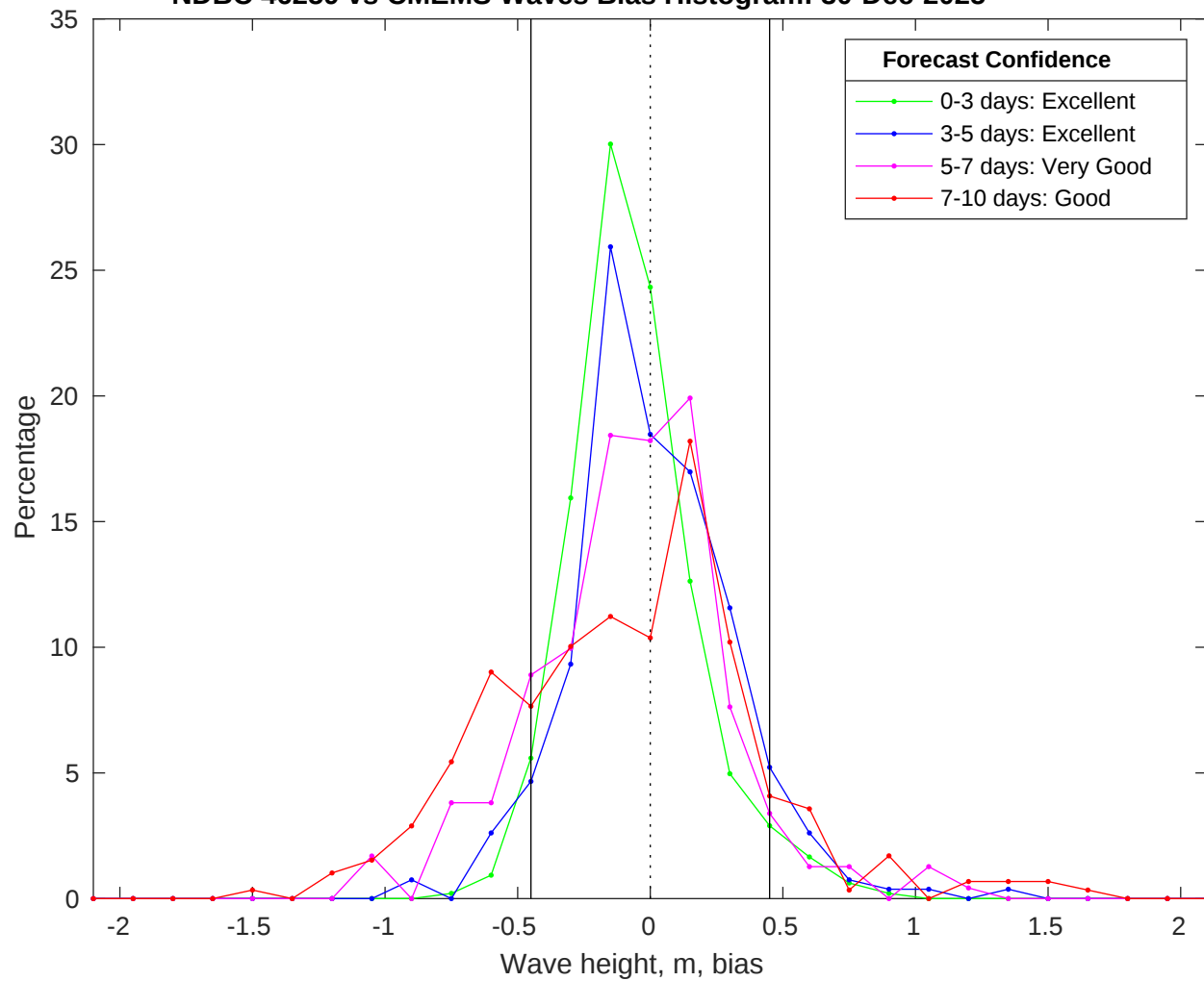
NDBC 46259 vs CMEMS Waves Bias Histogram: 30-Dec-2025
