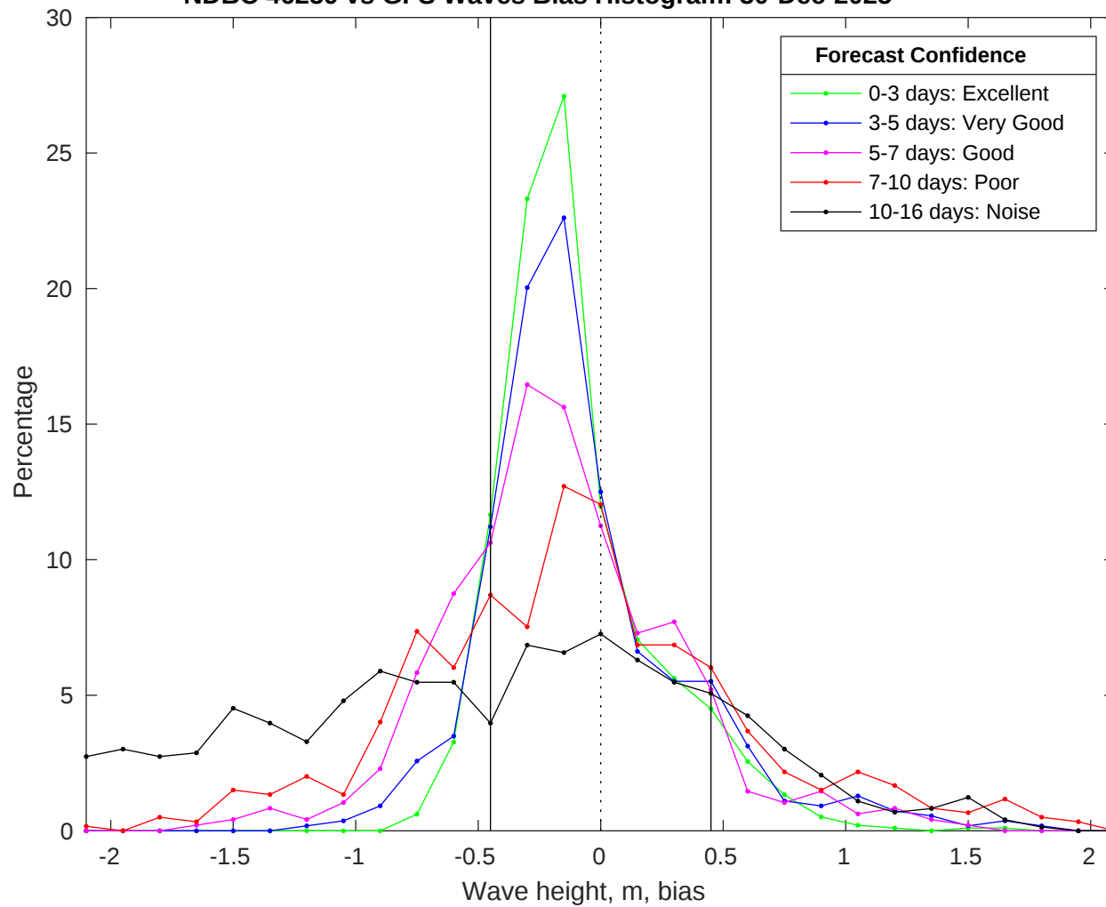
NDBC 46259 vs GFS Waves Bias Histogram: 30-Dec-2025
