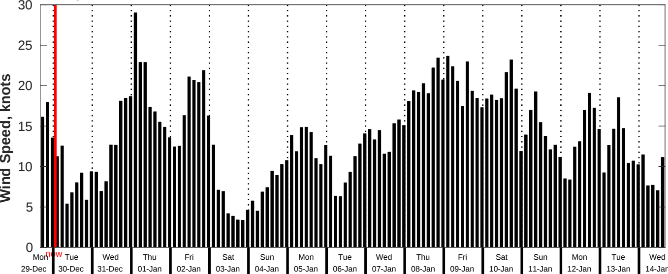
GFS Wind Speed Forecast for NDBC 46259 from 29-Dec-2025 16:00:00 to 14-Jan-2026 16:00:00
