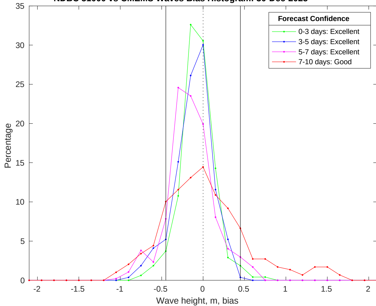
NDBC 51000 vs CMEMS Waves Bias Histogram: 30-Dec-2025
