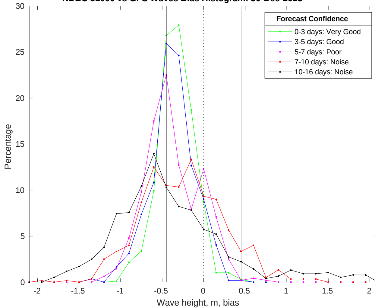
NDBC 51000 vs GFS Waves Bias Histogram: 30-Dec-2025
