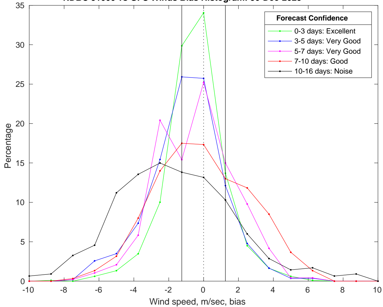
NDBC 51000 vs GFS Winds Bias Histogram: 30-Dec-2025
