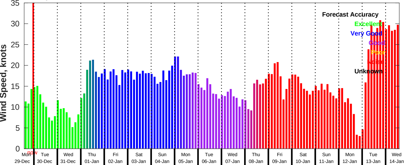
GFS Wind Speed Forecast for NDBC 51000 from 29-Dec-2025 14:00:00 to 14-Jan-2026 14:00:00
