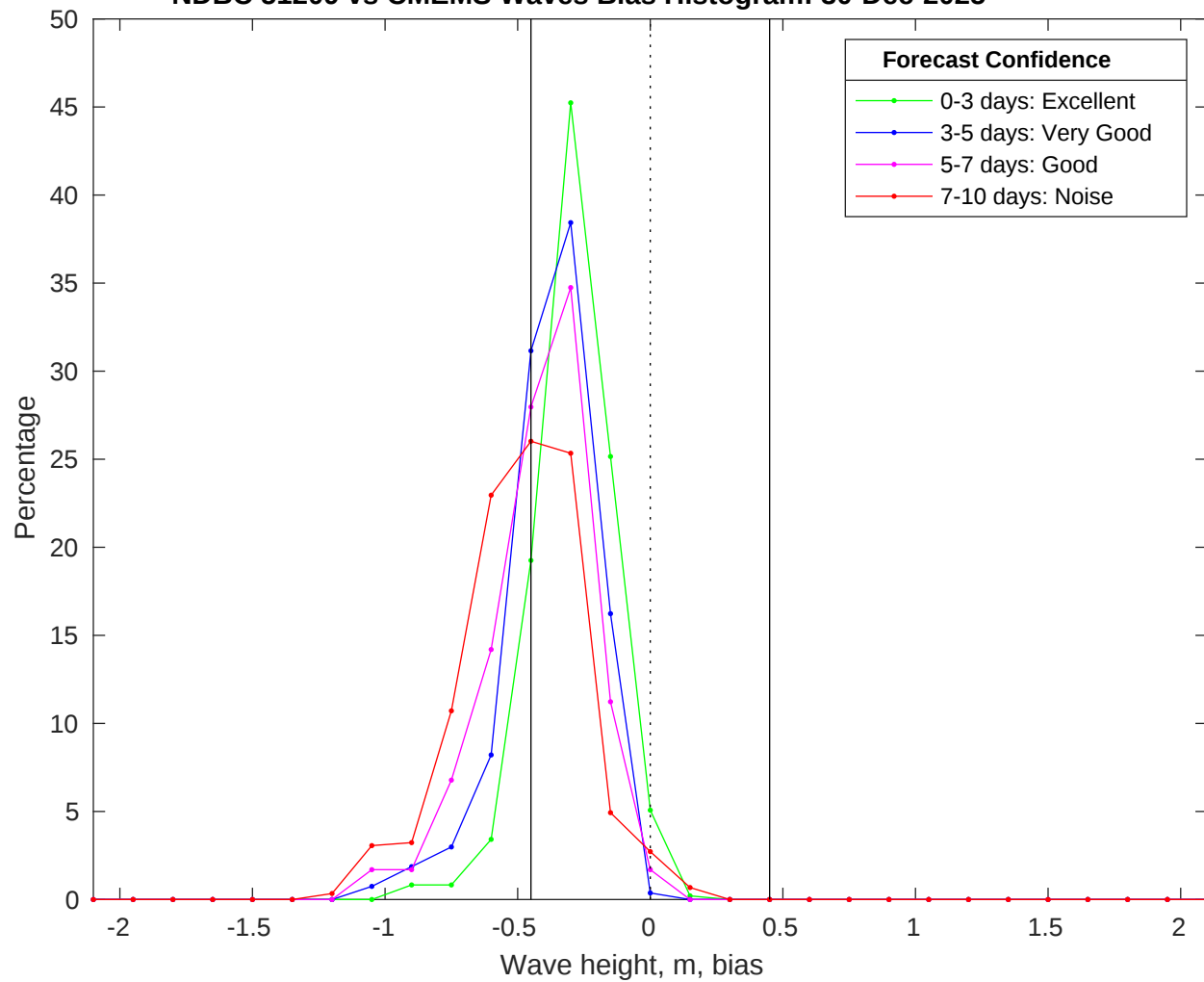
NDBC 51209 vs CMEMS Waves Bias Histogram: 30-Dec-2025
