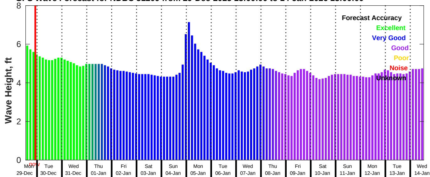
GFS Wave Forecast for NDBC 51209 from 29-Dec-2025 13:00:00 to 14-Jan-2026 13:00:00
