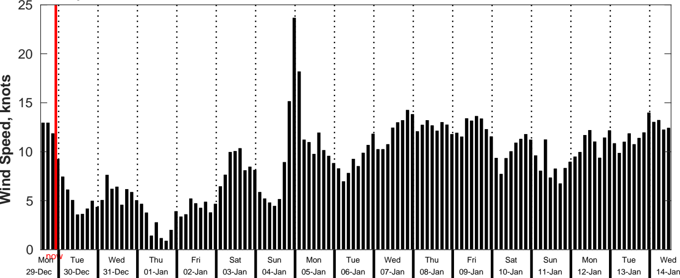
GFS Wind Speed Forecast for NDBC 51209 from 29-Dec-2025 13:00:00 to 14-Jan-2026 13:00:00
