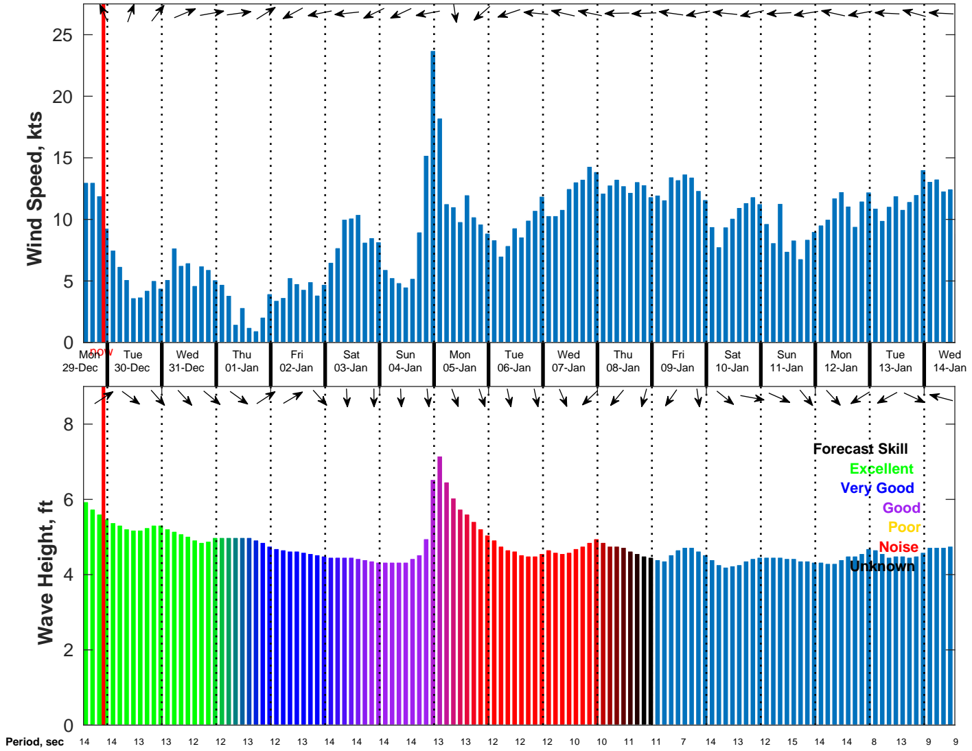
Wind & Wave Forecast for NDBC 51209 from 29-Dec-2025 13:00:00 to 14-Jan-2026 13:00:00
