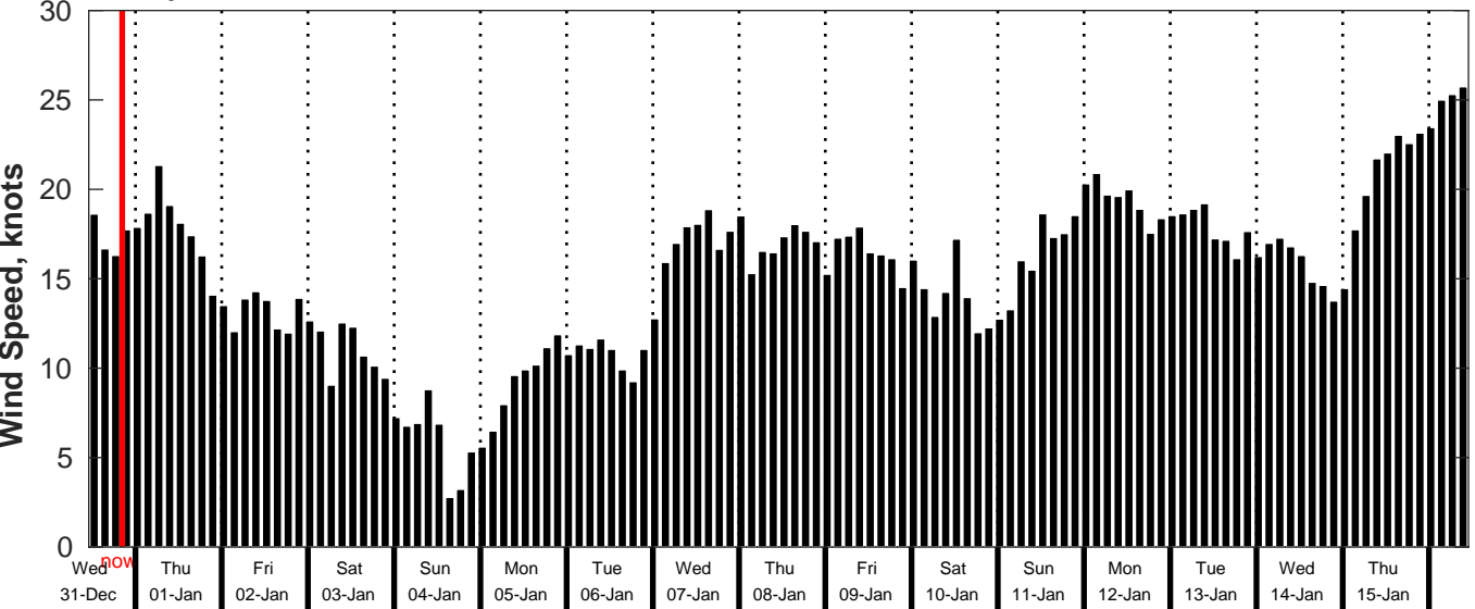
GFS Wind Speed Forecast for NDBC 52211 from 30-Dec-2025 11:00:00 to 15-Jan-2026 11:00:00
