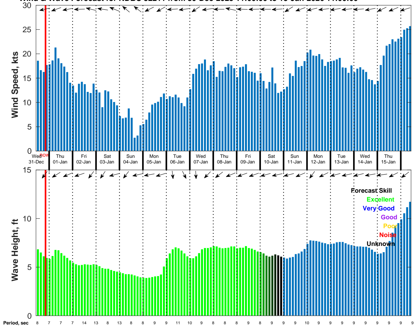
Wind & Wave Forecast for NDBC 52211 from 30-Dec-2025 11:00:00 to 15-Jan-2026 11:00:00
