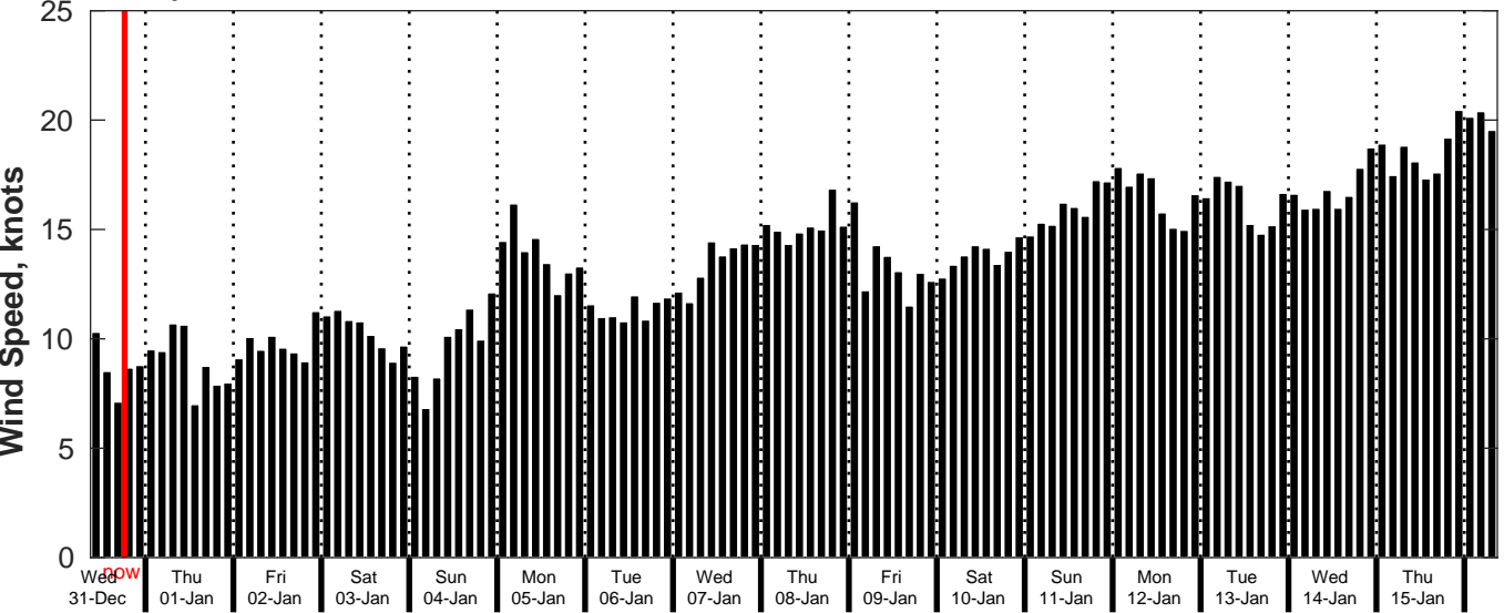
GFS Wind Speed Forecast for NDBC 52212 from 30-Dec-2025 09:00:00 to 15-Jan-2026 09:00:00
