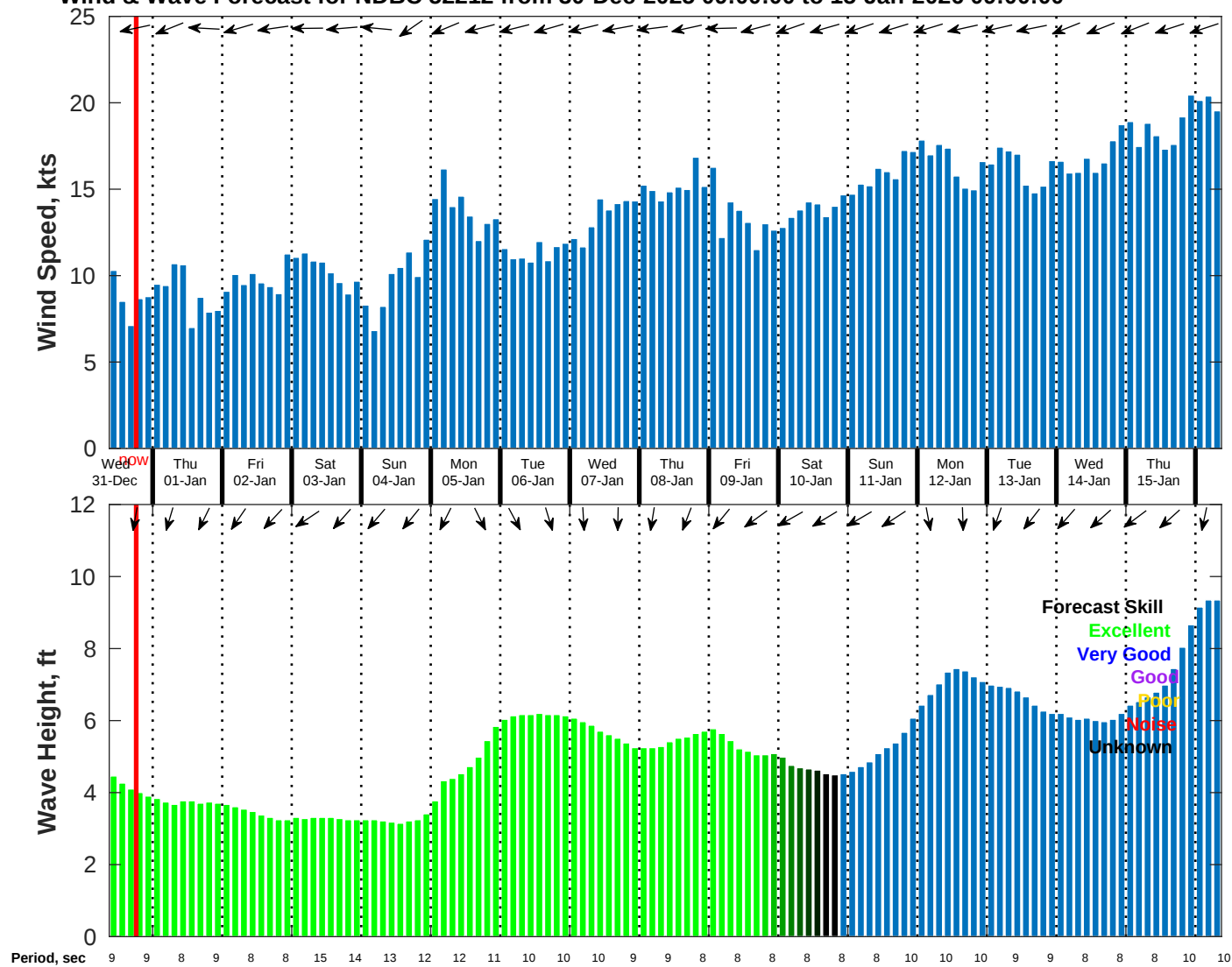
Wind & Wave Forecast for NDBC 52212 from 30-Dec-2025 09:00:00 to 15-Jan-2026 09:00:00
