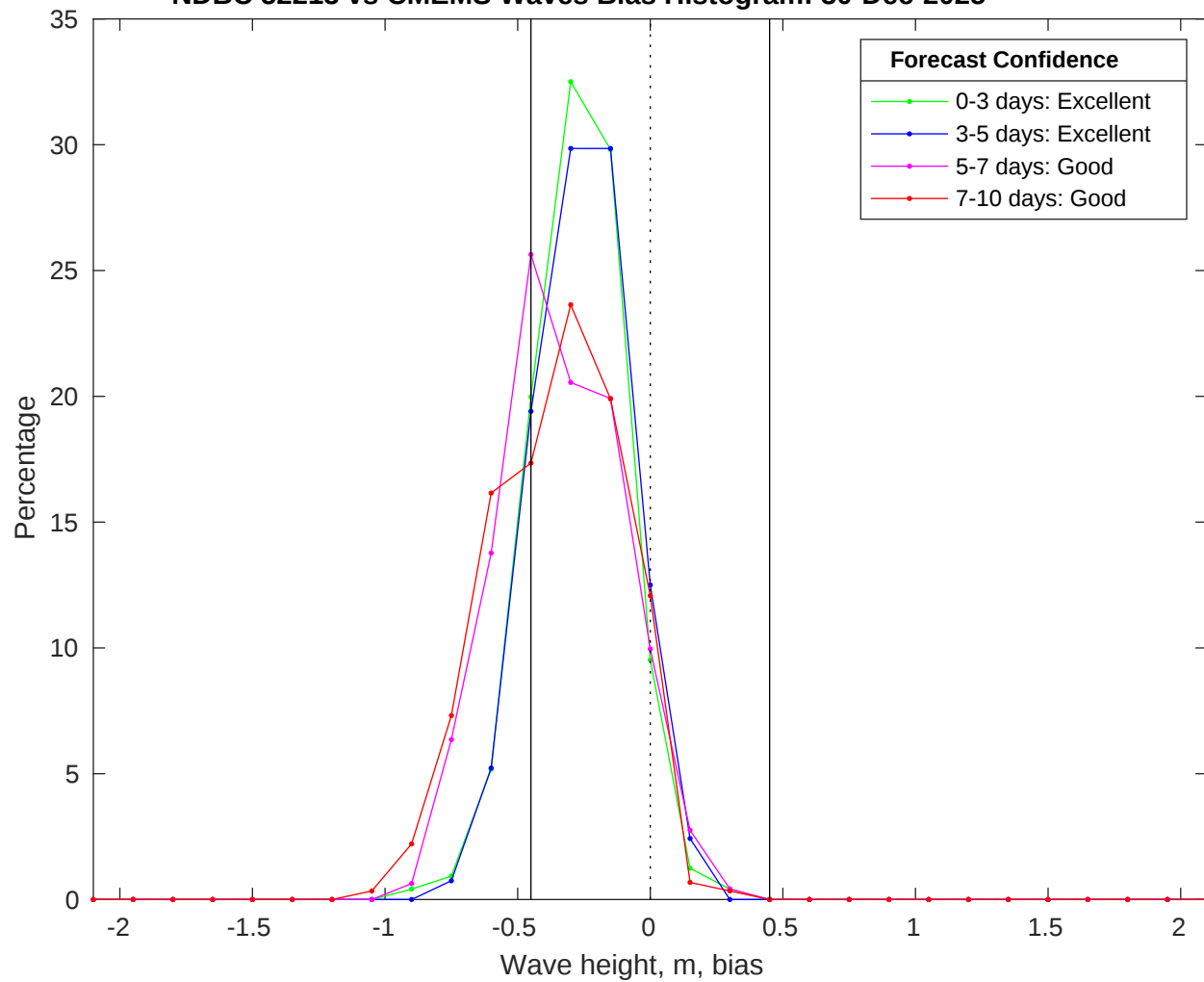
NDBC 52213 vs CMEMS Waves Bias Histogram: 30-Dec-2025
