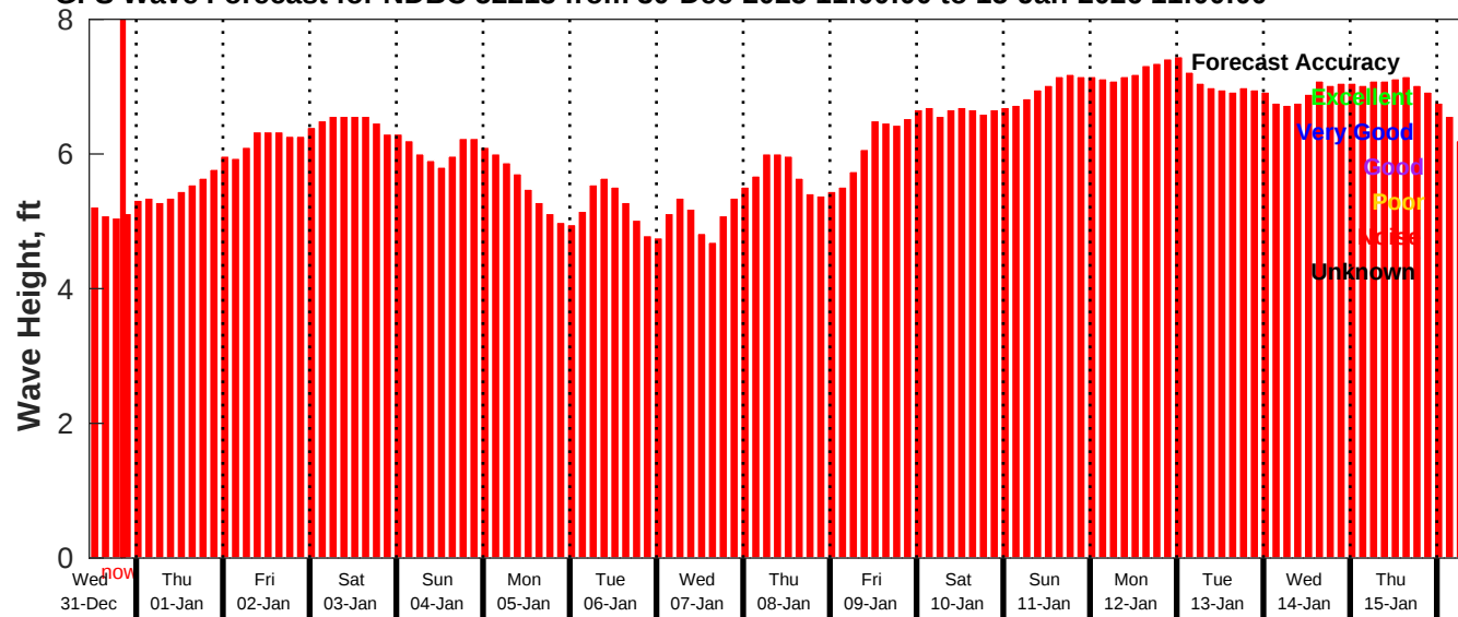
GFS Wave Forecast for NDBC 52213 from 30-Dec-2025 11:00:00 to 15-Jan-2026 11:00:00
