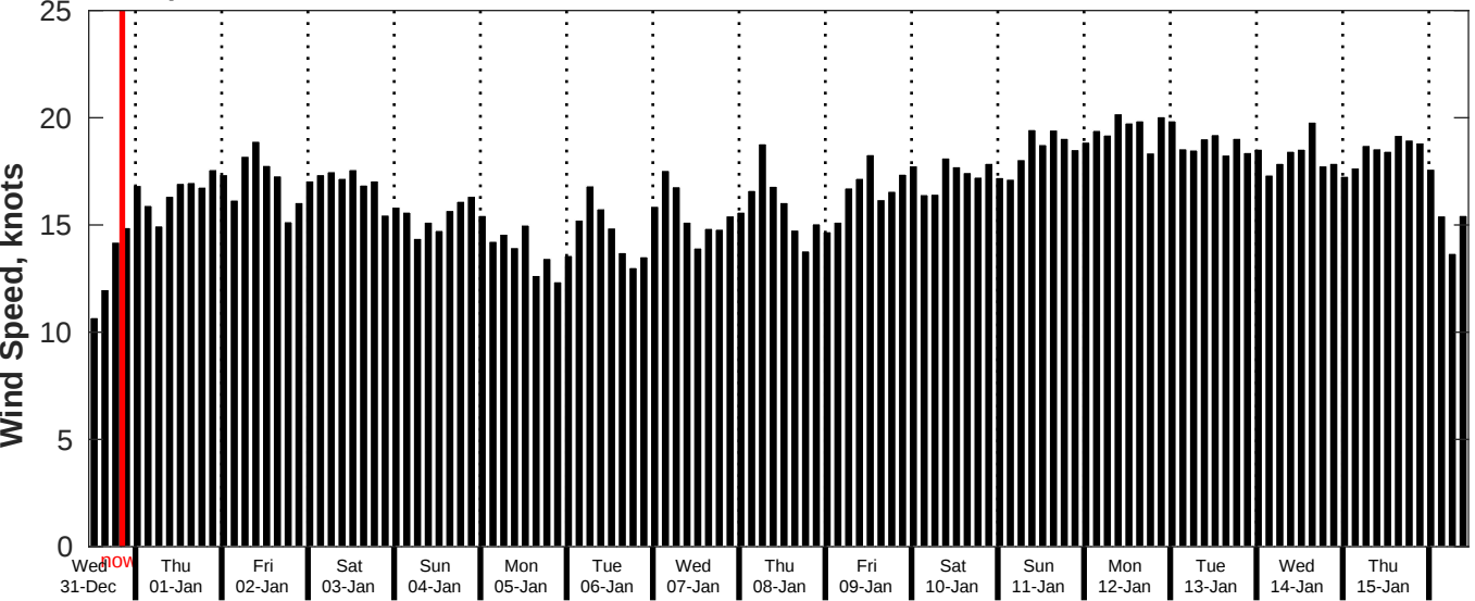
GFS Wind Speed Forecast for NDBC 52213 from 30-Dec-2025 11:00:00 to 15-Jan-2026 11:00:00
