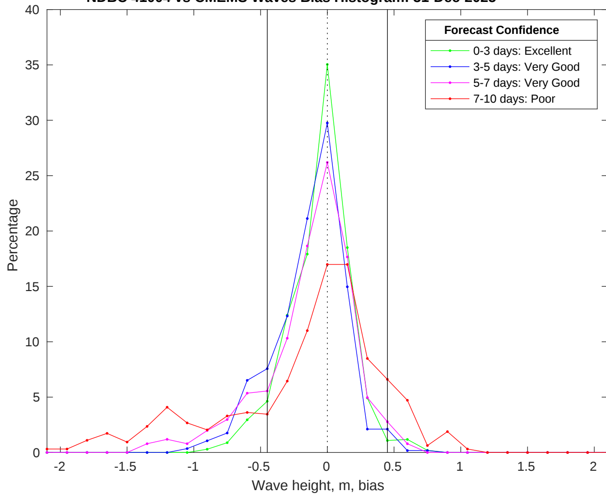
NDBC 41004 vs CMEMS Waves Bias Histogram: 31-Dec-2025
