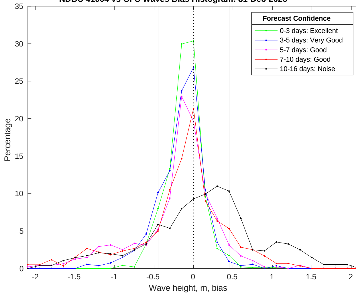
NDBC 41004 vs GFS Waves Bias Histogram: 31-Dec-2025
