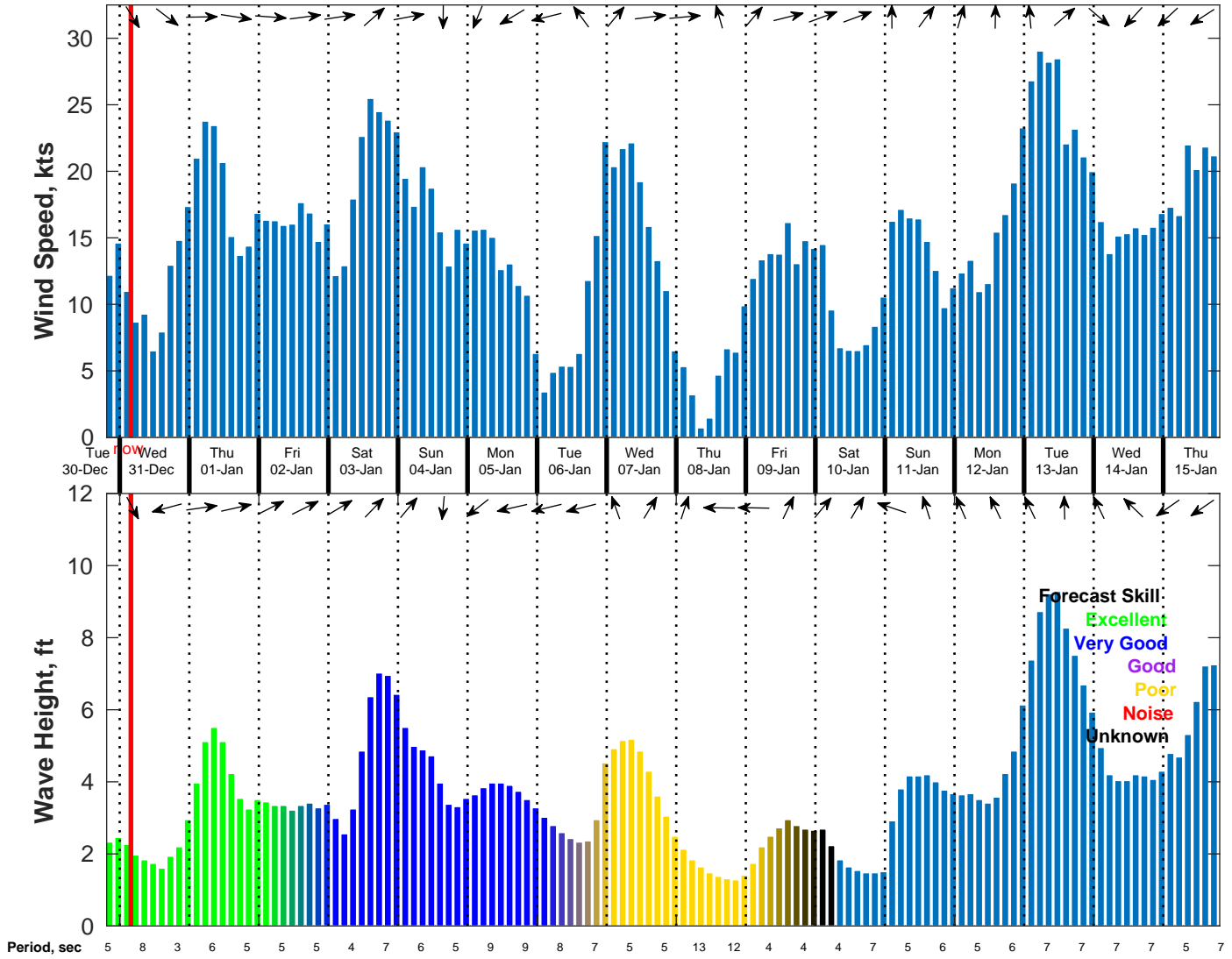
Wind & Wave Forecast for NDBC 41004 from 30-Dec-2025 19:00:00 to 15-Jan-2026 19:00:00
