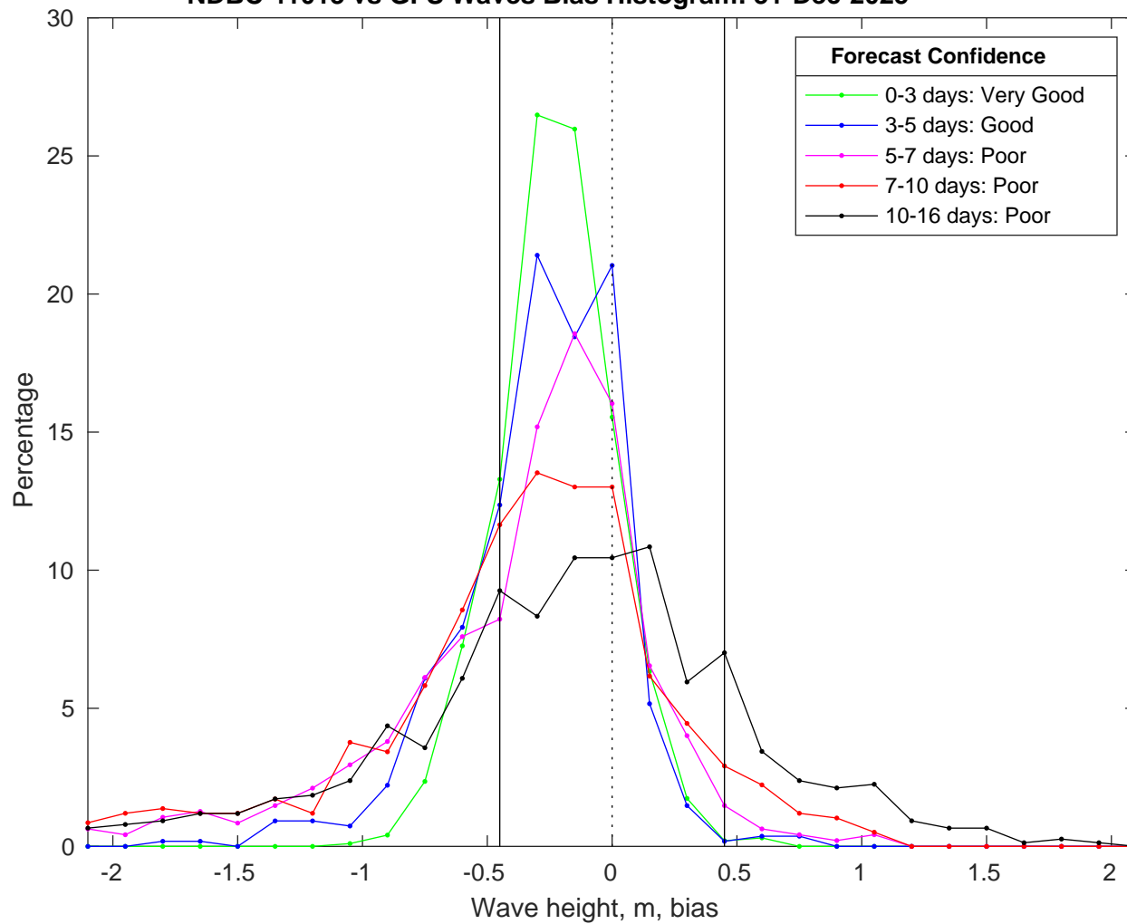
NDBC 41013 vs GFS Waves Bias Histogram: 31-Dec-2025
