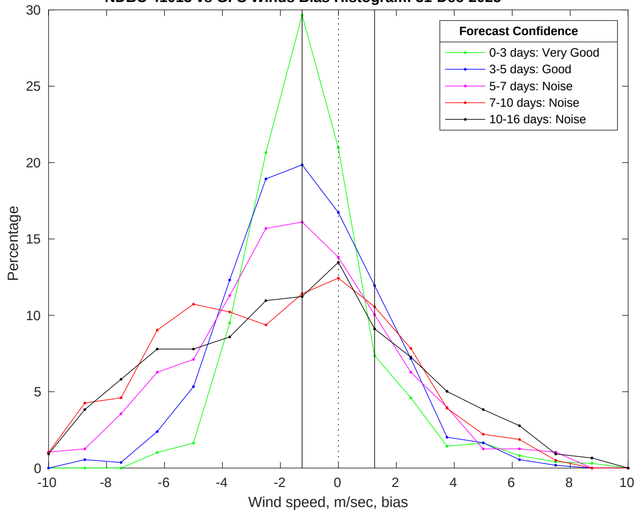
NDBC 41013 vs GFS Winds Bias Histogram: 31-Dec-2025
