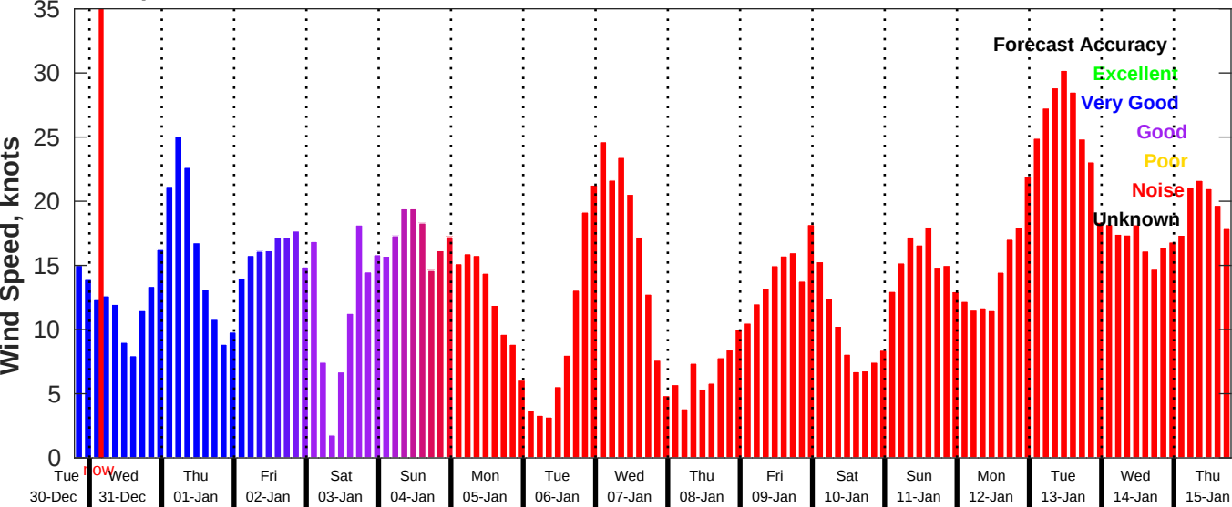
GFS Wind Speed Forecast for NDBC 41013 from 30-Dec-2025 19:00:00 to 15-Jan-2026 19:00:00
