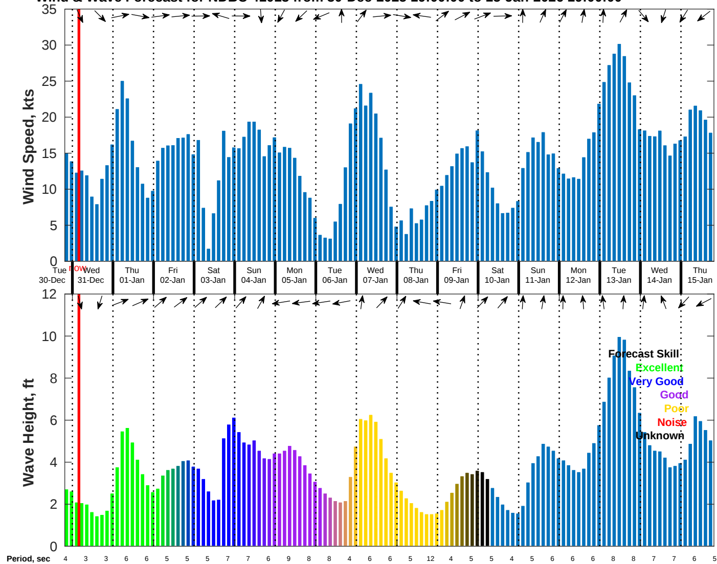
Wind & Wave Forecast for NDBC 41013 from 30-Dec-2025 19:00:00 to 15-Jan-2026 19:00:00
