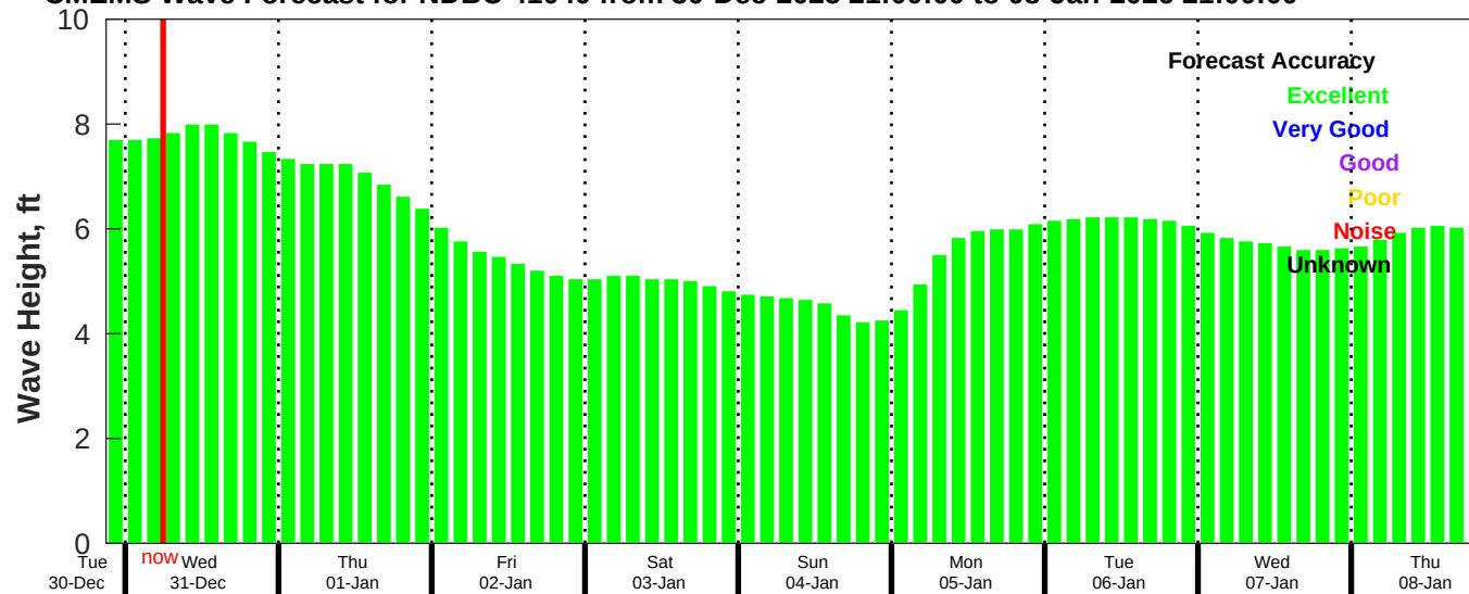
CMEMS Wave Forecast for NDBC 41040 from 30-Dec-2025 21:00:00 to 08-Jan-2026 21:00:00
