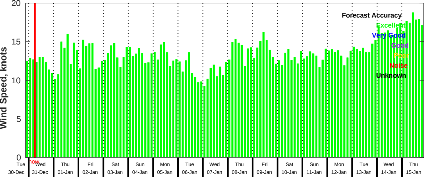
GFS Wind Speed Forecast for NDBC 41040 from 30-Dec-2025 21:00:00 to 15-Jan-2026 21:00:00
