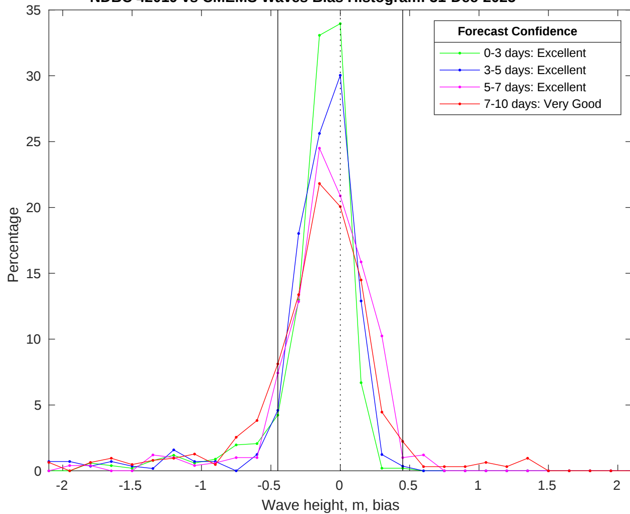
NDBC 42019 vs CMEMS Waves Bias Histogram: 31-Dec-2025
