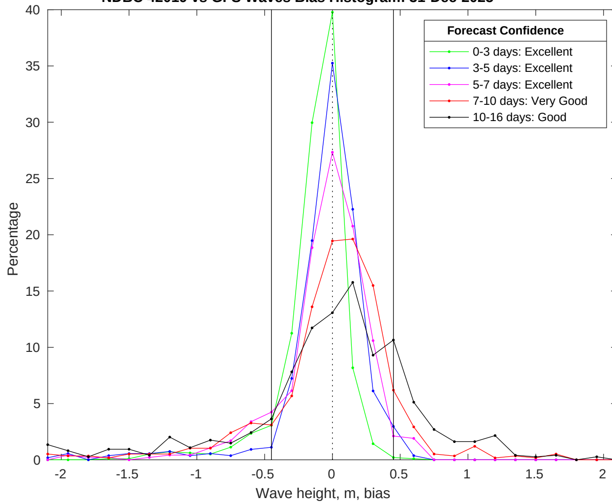
NDBC 42019 vs GFS Waves Bias Histogram: 31-Dec-2025
