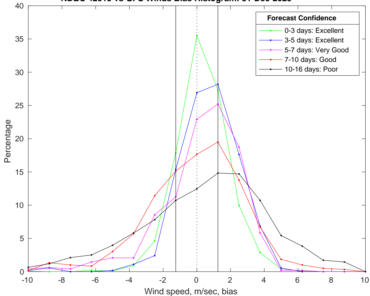
NDBC 42019 vs GFS Winds Bias Histogram: 31-Dec-2025
