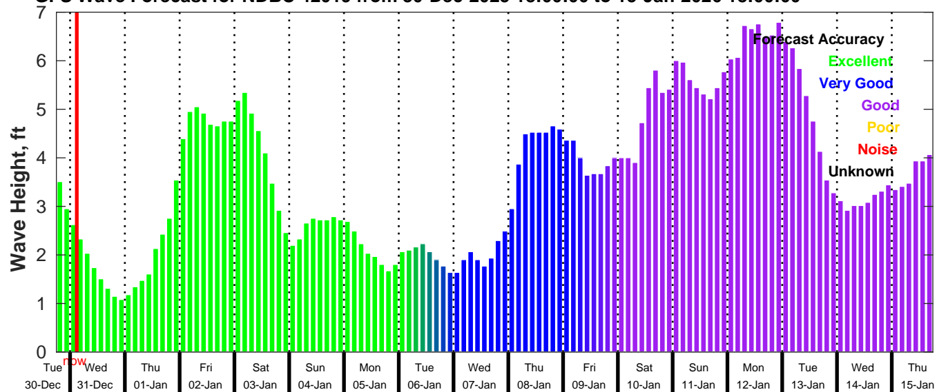
GFS Wave Forecast for NDBC 42019 from 30-Dec-2025 18:00:00 to 15-Jan-2026 18:00:00
