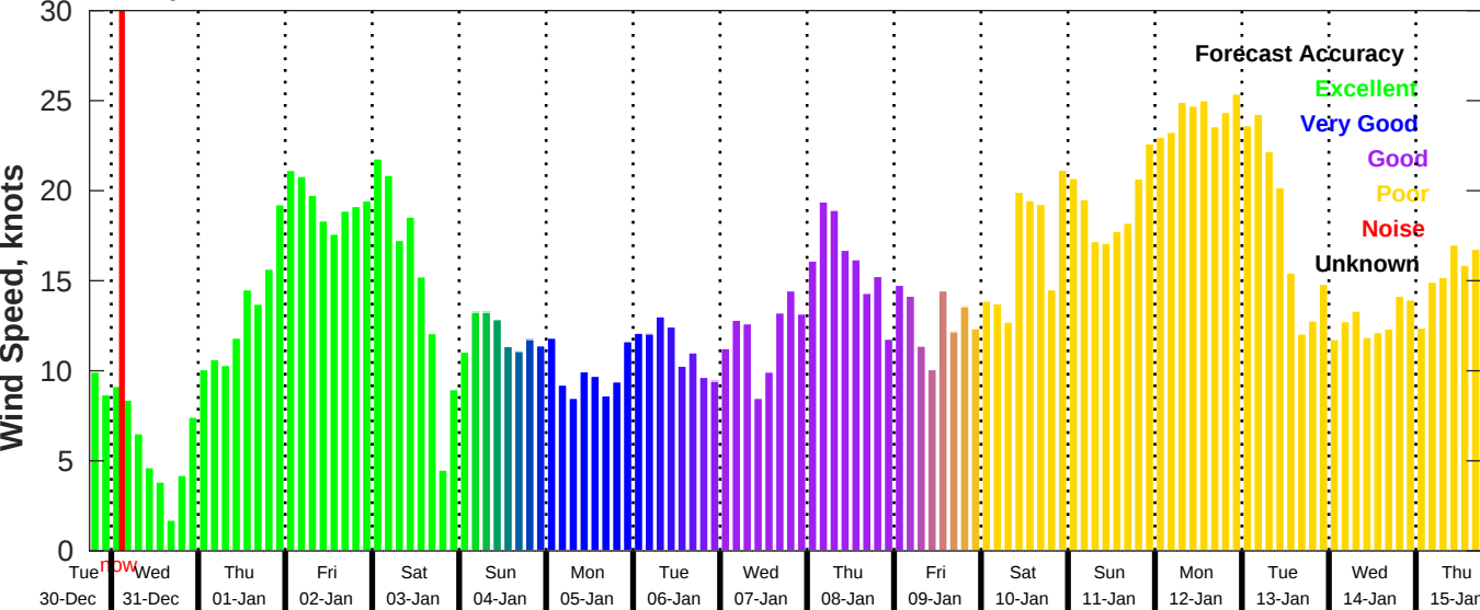
GFS Wind Speed Forecast for NDBC 42019 from 30-Dec-2025 18:00:00 to 15-Jan-2026 18:00:00
