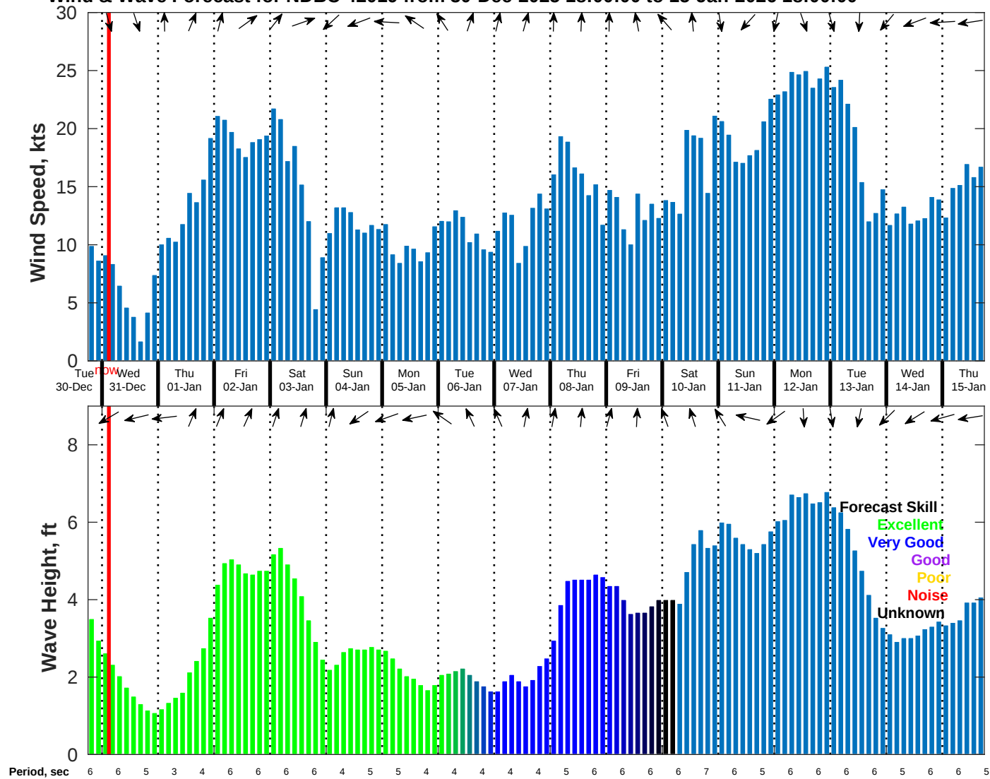
Wind & Wave Forecast for NDBC 42019 from 30-Dec-2025 18:00:00 to 15-Jan-2026 18:00:00
