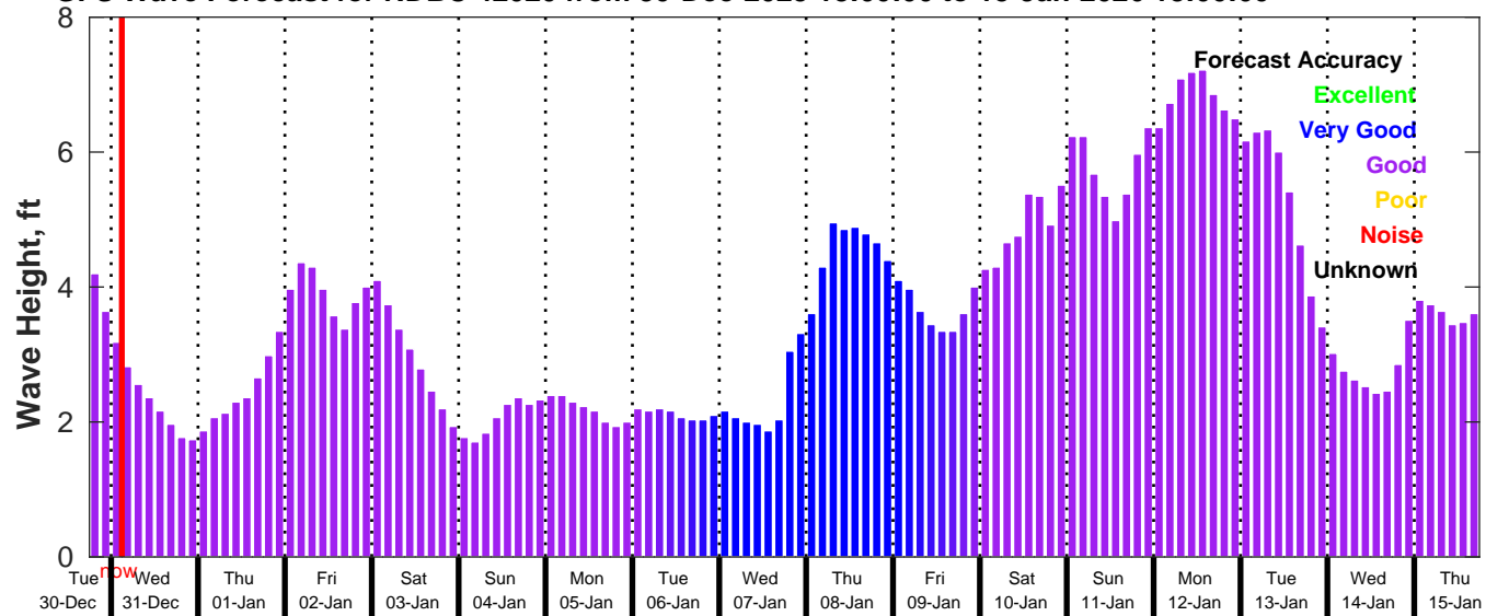
GFS Wave Forecast for NDBC 42020 from 30-Dec-2025 18:00:00 to 15-Jan-2026 18:00:00
