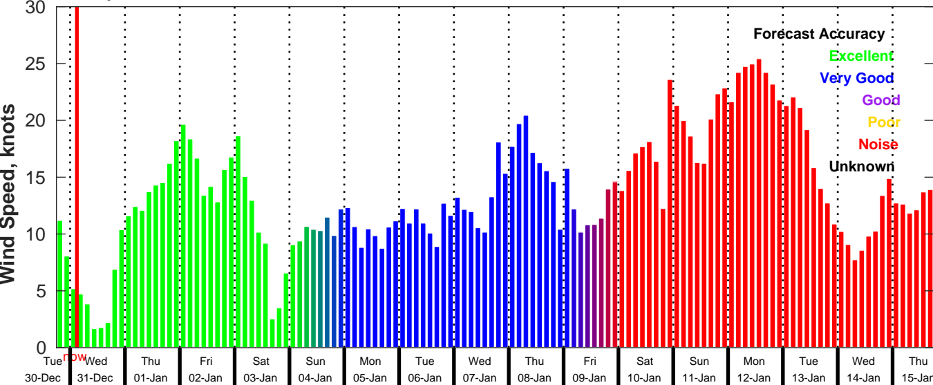
GFS Wind Speed Forecast for NDBC 42020 from 30-Dec-2025 18:00:00 to 15-Jan-2026 18:00:00
