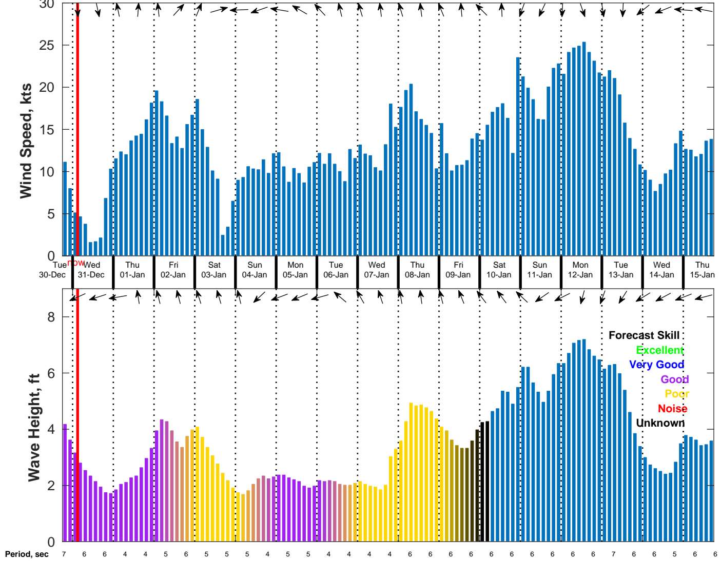
Wind & Wave Forecast for NDBC 42020 from 30-Dec-2025 18:00:00 to 15-Jan-2026 18:00:00
