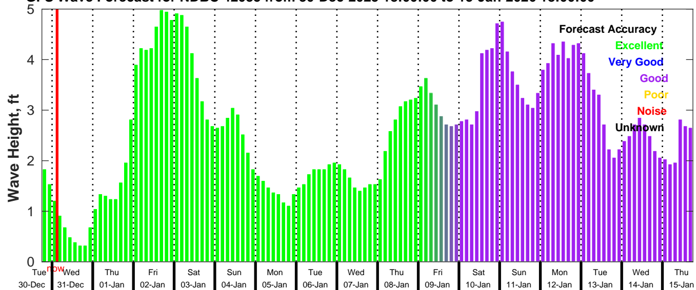
GFS Wave Forecast for NDBC 42035 from 30-Dec-2025 18:00:00 to 15-Jan-2026 18:00:00
