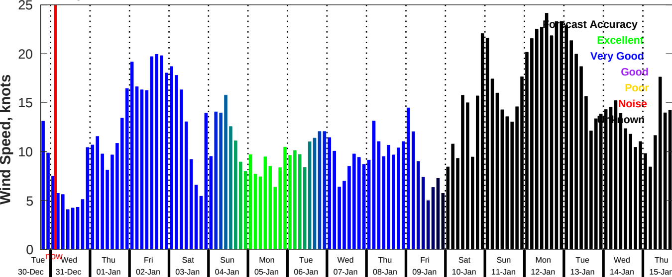
GFS Wind Speed Forecast for NDBC 42035 from 30-Dec-2025 18:00:00 to 15-Jan-2026 18:00:00
