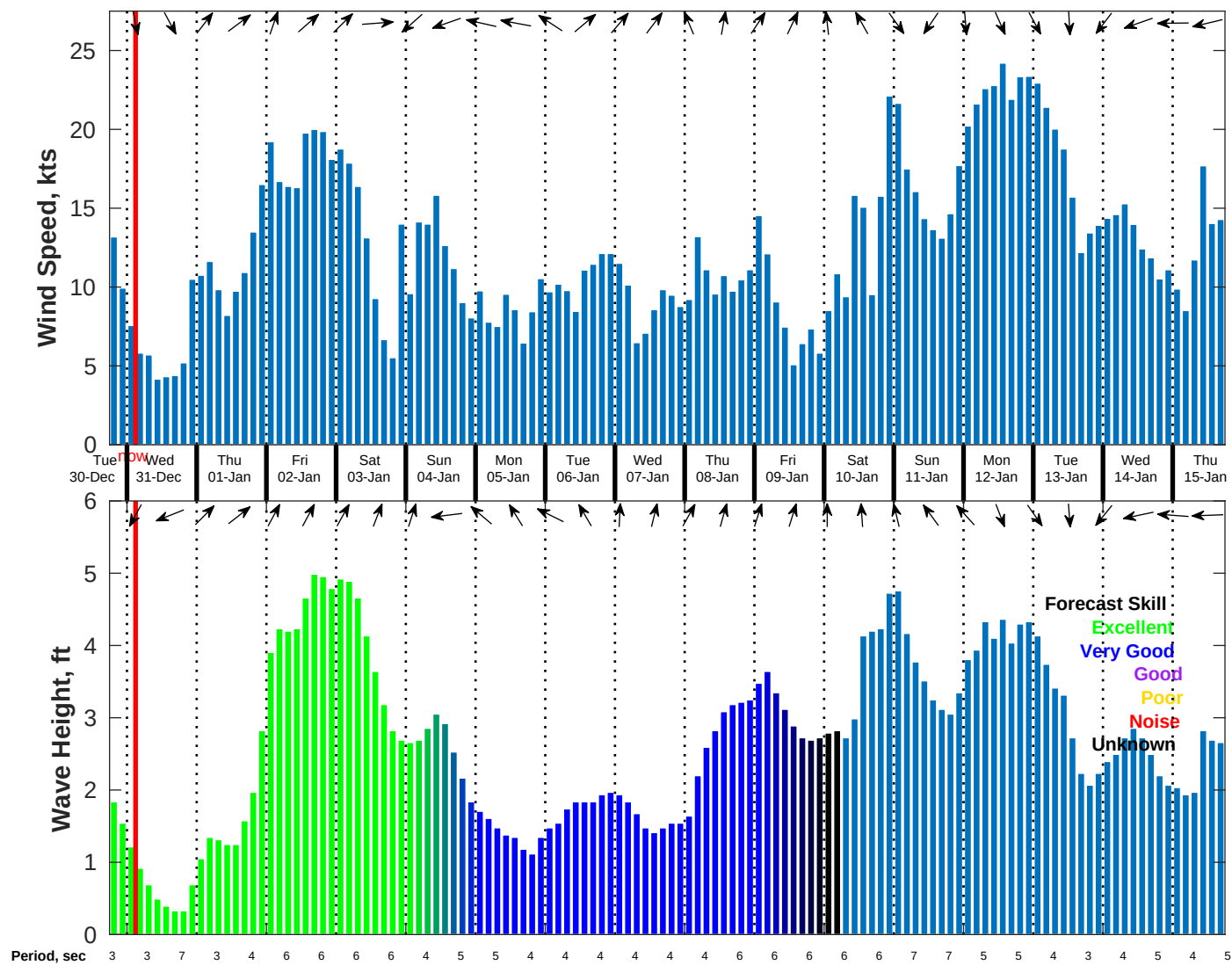
Wind & Wave Forecast for NDBC 42035 from 30-Dec-2025 18:00:00 to 15-Jan-2026 18:00:00
