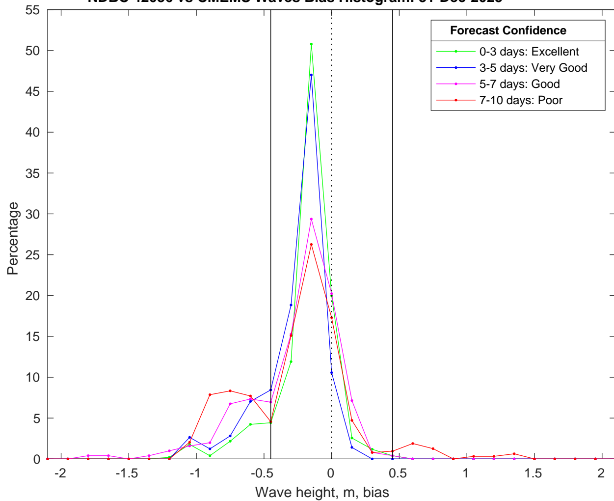
NDBC 42036 vs CMEMS Waves Bias Histogram: 31-Dec-2025
