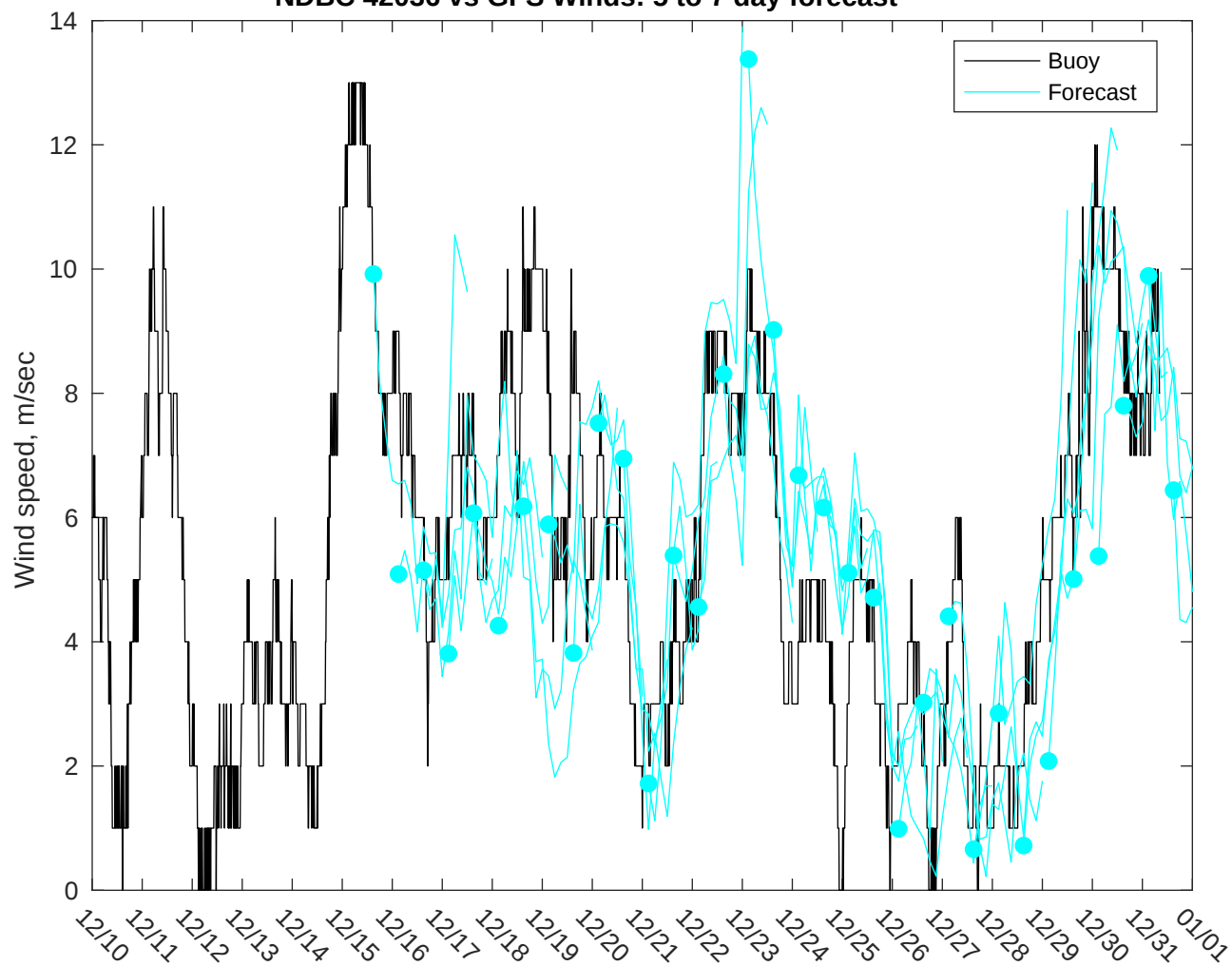
NDBC 42036 vs GFS Winds: 5 to 7 day forecast
