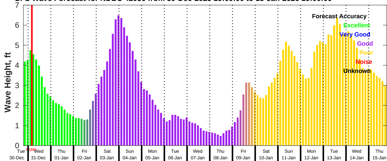
GFS Wave Forecast for NDBC 42036 from 30-Dec-2025 19:00:00 to 15-Jan-2026 19:00:00
