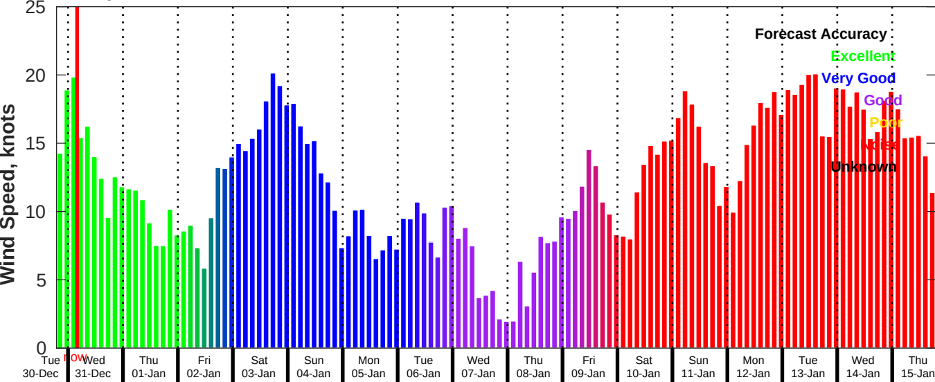
GFS Wind Speed Forecast for NDBC 42036 from 30-Dec-2025 19:00:00 to 15-Jan-2026 19:00:00
